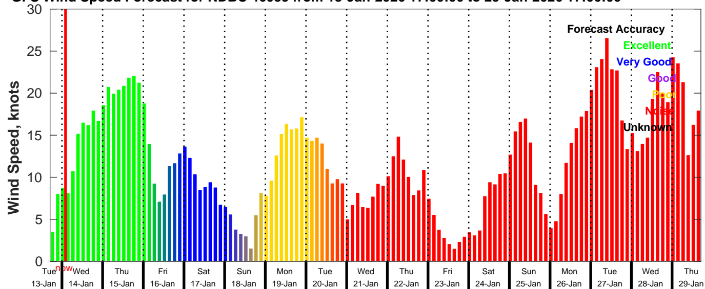
GFS Wind Speed Forecast for NDBC 46059 from 13-Jan-2026 17:00:00 to 29-Jan-2026 17:00:00
