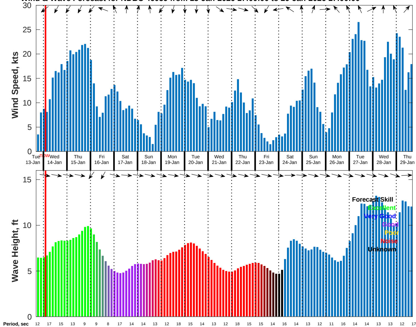
Wind & Wave Forecast for NDBC 46059 from 13-Jan-2026 17:00:00 to 29-Jan-2026 17:00:00
