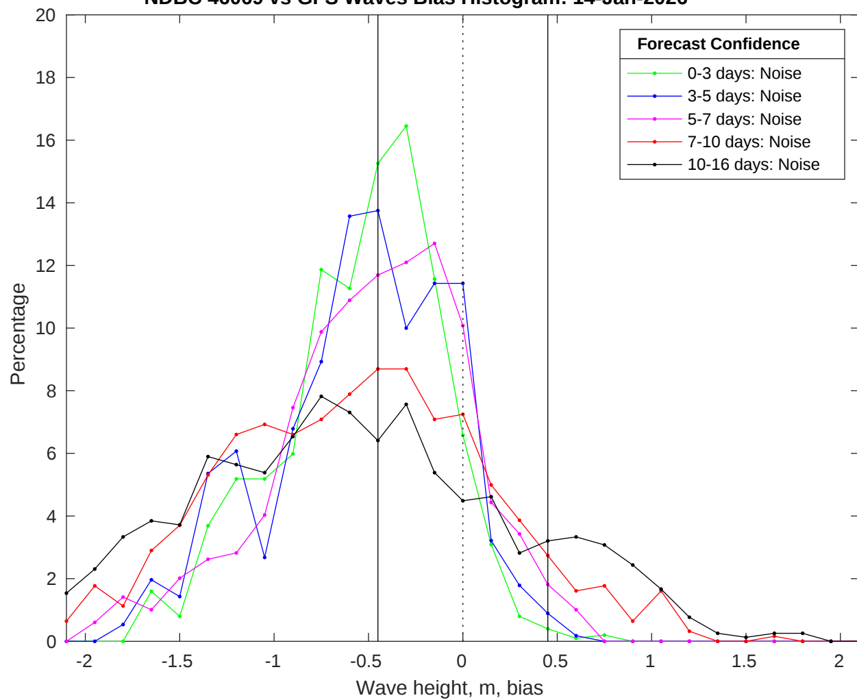
NDBC 46069 vs GFS Waves Bias Histogram: 14-Jan-2026
