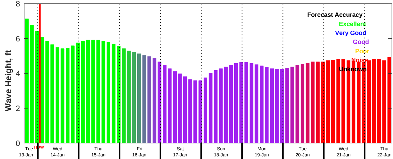
CMEMS Wave Forecast for NDBC 46069 from 13-Jan-2026 16:00:00 to 22-Jan-2026 16:00:00
