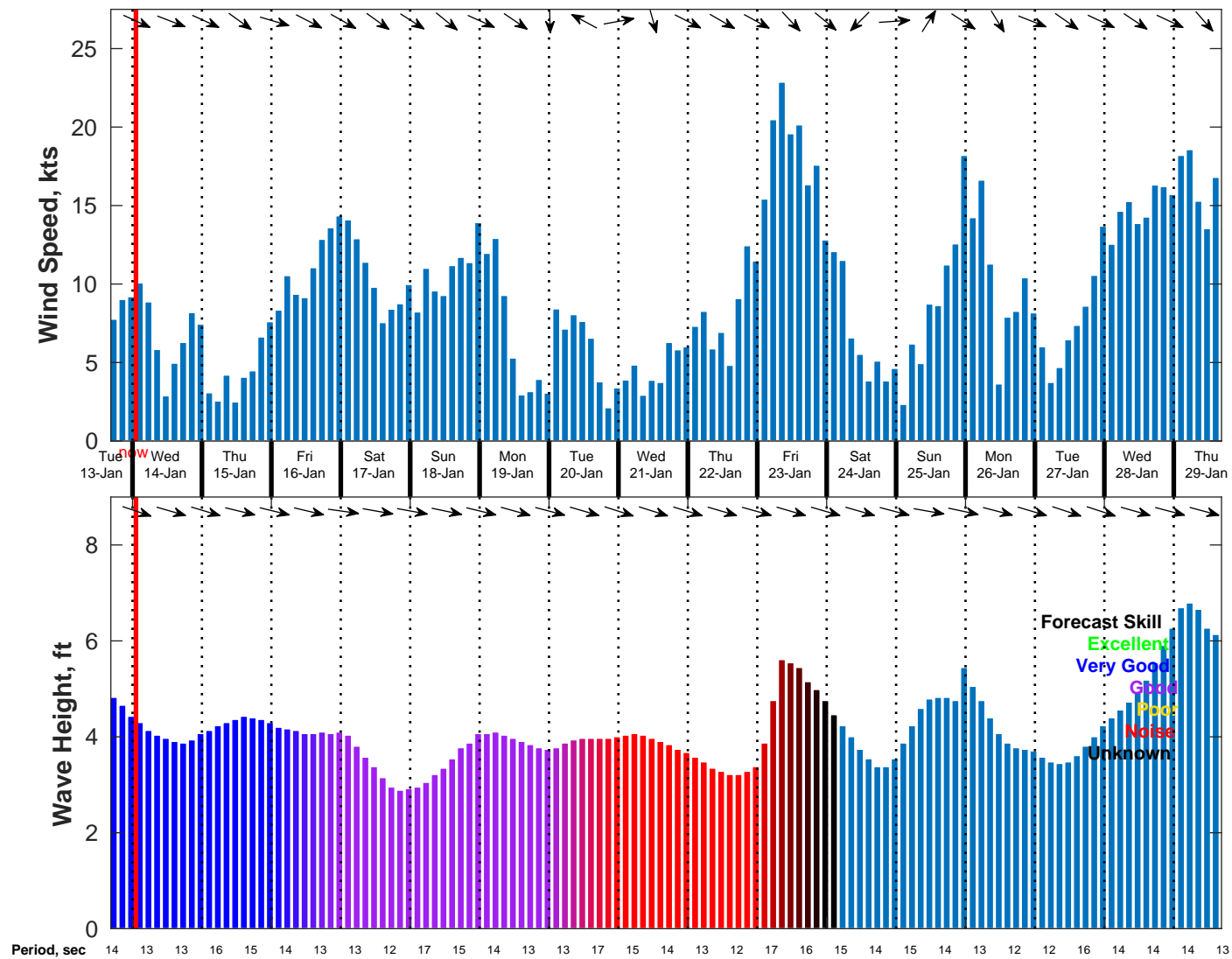
Wind & Wave Forecast for NDBC 46069 from 13-Jan-2026 16:00:00 to 29-Jan-2026 16:00:00
