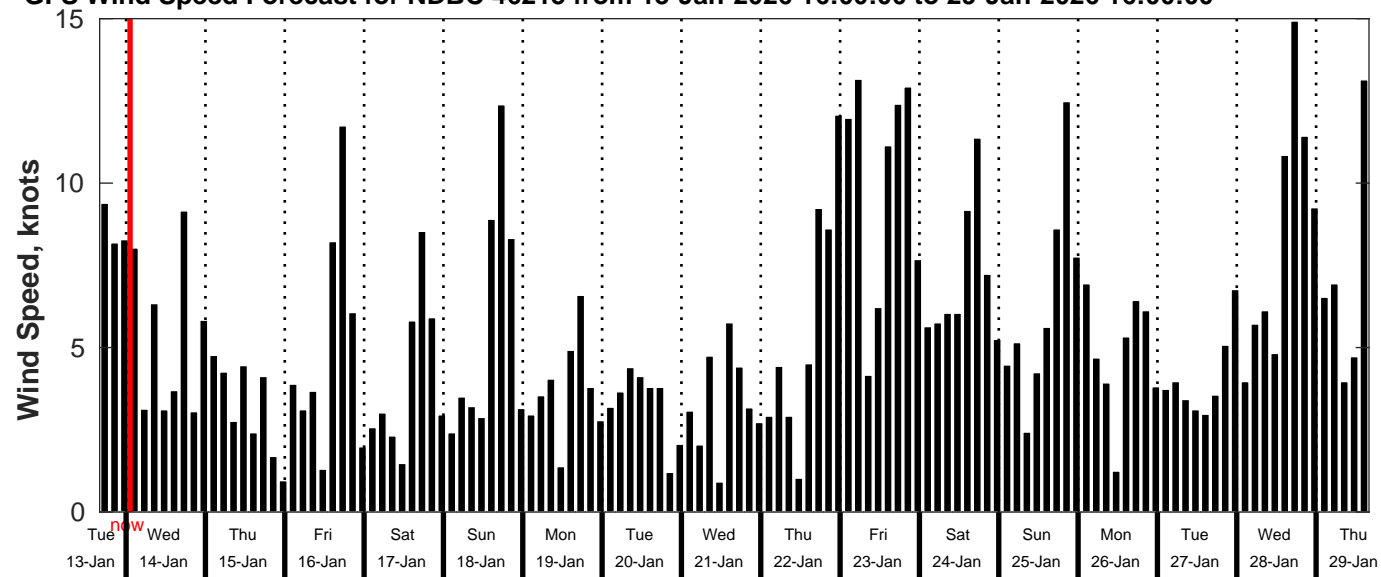
GFS Wind Speed Forecast for NDBC 46215 from 13-Jan-2026 16:00:00 to 29-Jan-2026 16:00:00
