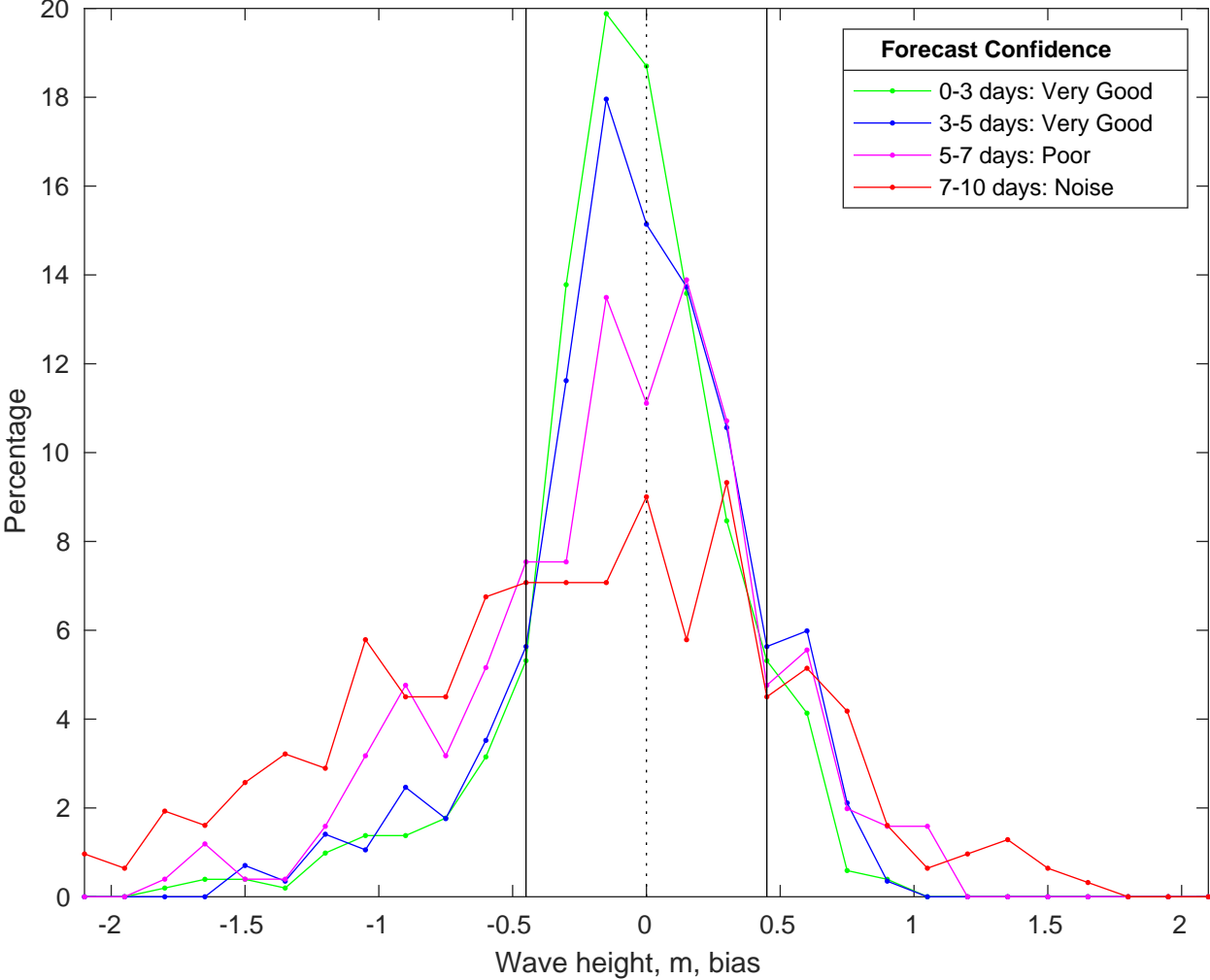
NDBC 46259 vs CMEMS Waves Bias Histogram: 14-Jan-2026
