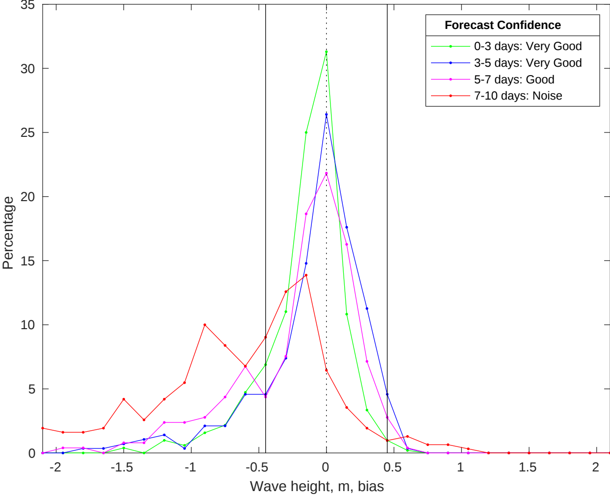
NDBC 51000 vs CMEMS Waves Bias Histogram: 14-Jan-2026
