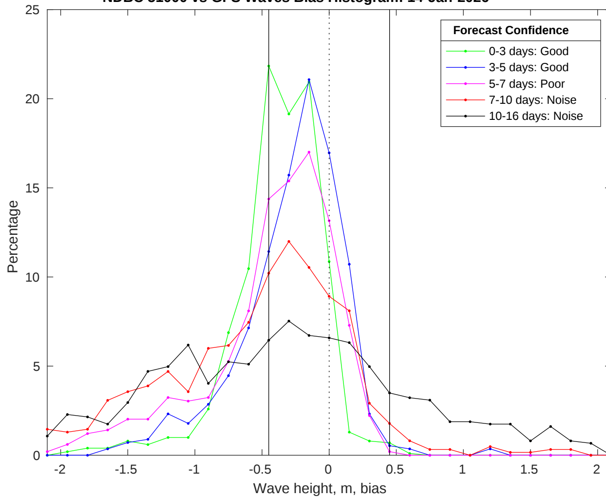
NDBC 51000 vs GFS Waves Bias Histogram: 14-Jan-2026
