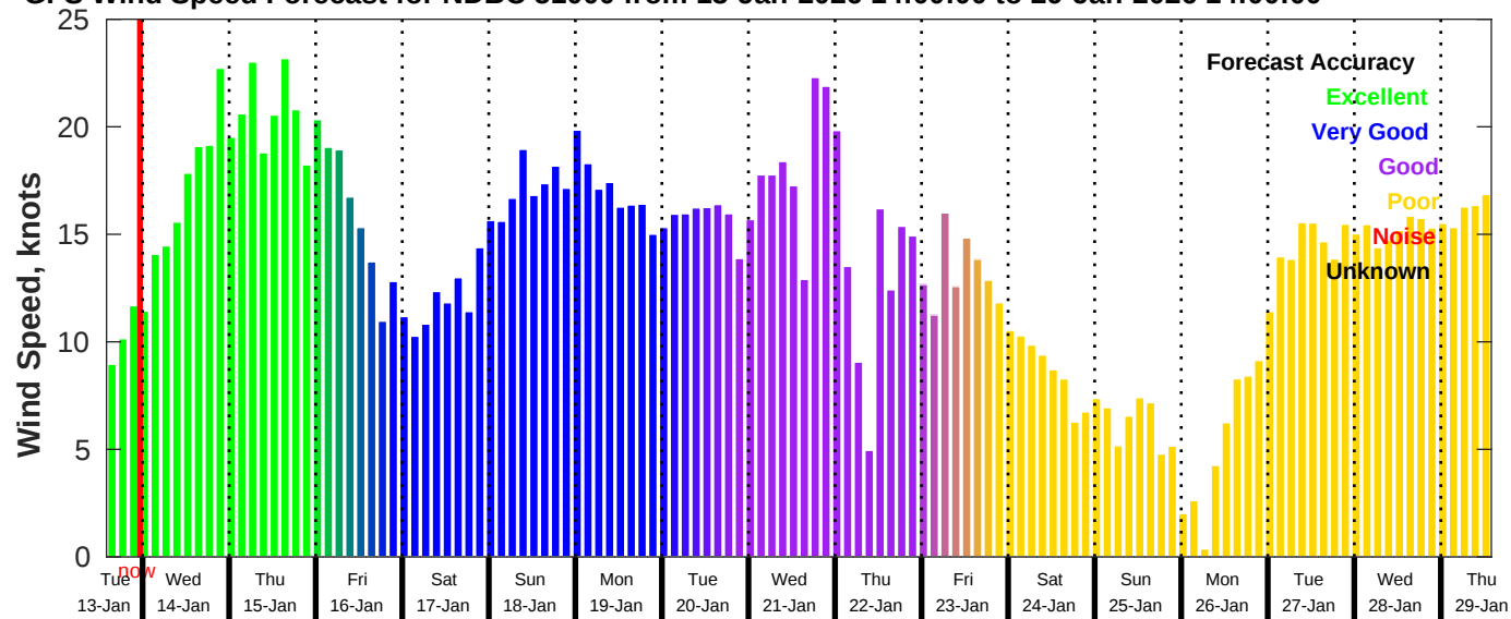
GFS Wind Speed Forecast for NDBC 51000 from 13-Jan-2026 14:00:00 to 29-Jan-2026 14:00:00
