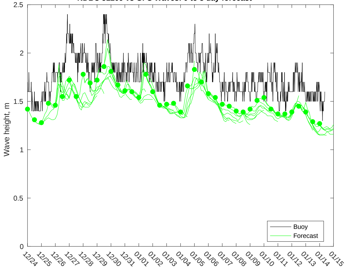
NDBC 51209 vs GFS Waves: 0 to 3 day forecast
