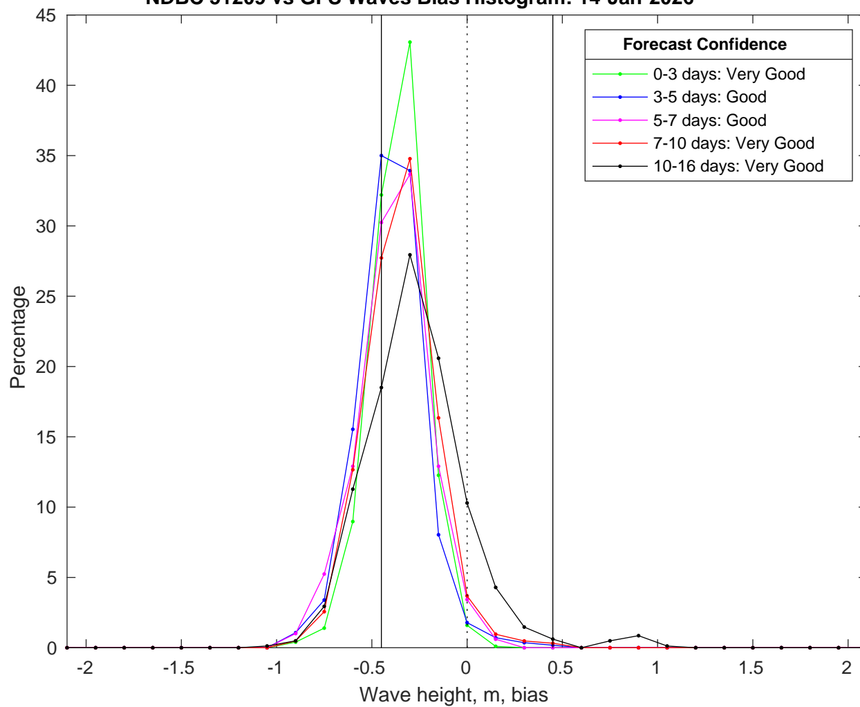
NDBC 51209 vs GFS Waves Bias Histogram: 14-Jan-2026
