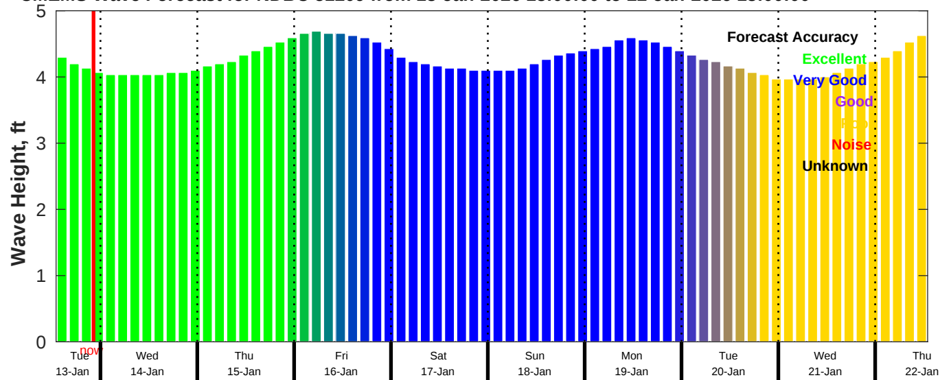
CMEMS Wave Forecast for NDBC 51209 from 13-Jan-2026 13:00:00 to 22-Jan-2026 13:00:00
