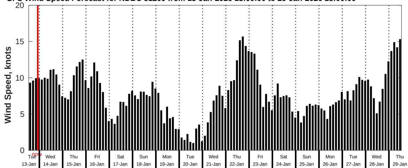
GFS Wind Speed Forecast for NDBC 51209 from 13-Jan-2026 13:00:00 to 29-Jan-2026 13:00:00
