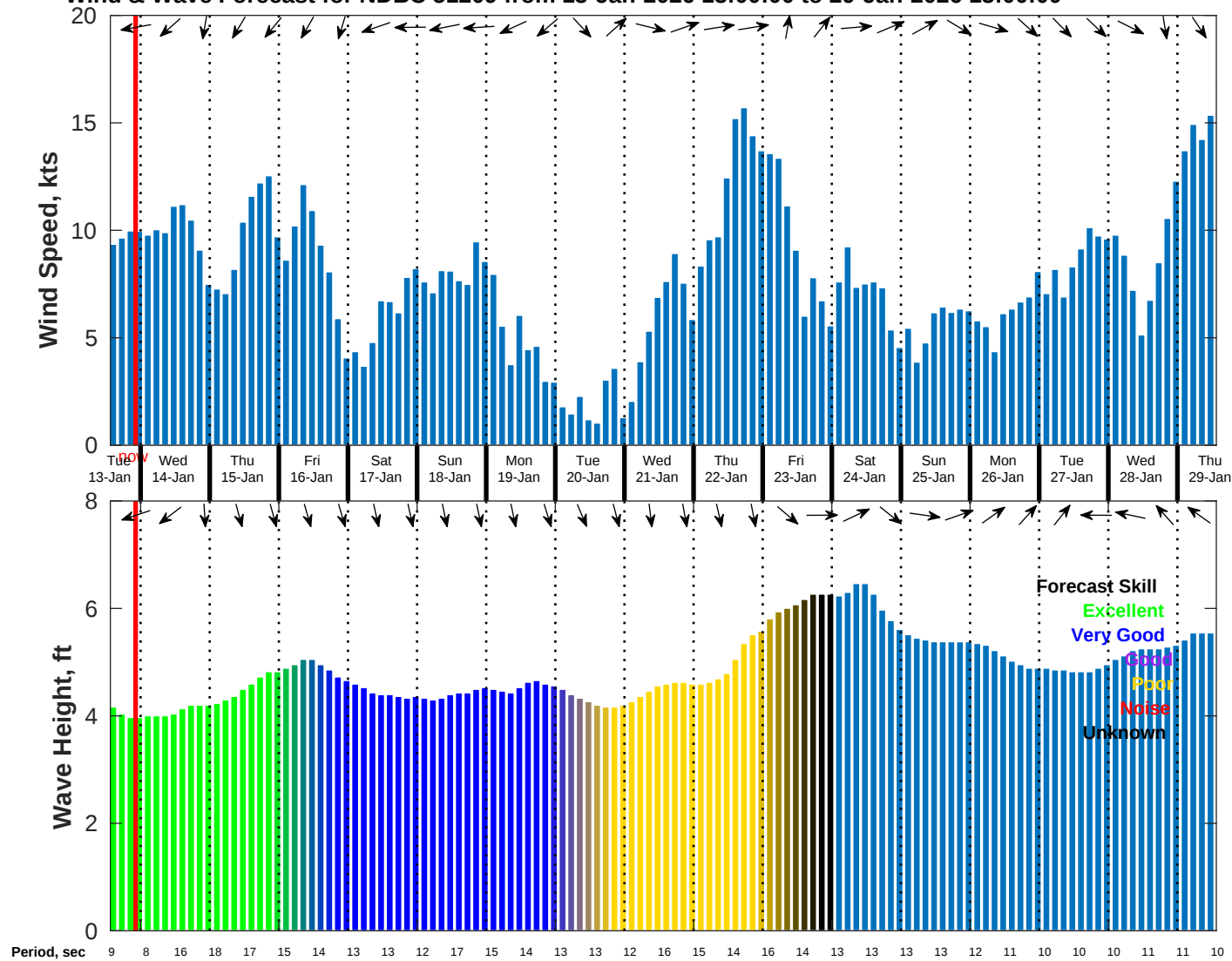
Wind & Wave Forecast for NDBC 51209 from 13-Jan-2026 13:00:00 to 29-Jan-2026 13:00:00
