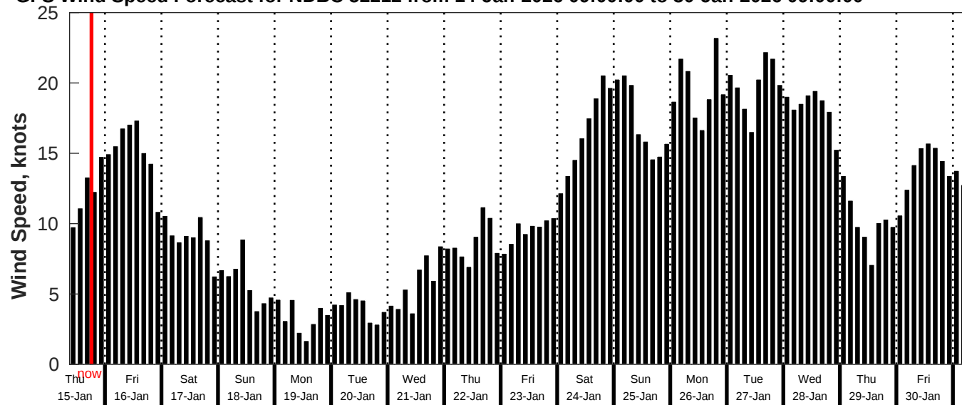
GFS Wind Speed Forecast for NDBC 52212 from 14-Jan-2026 09:00:00 to 30-Jan-2026 09:00:00
