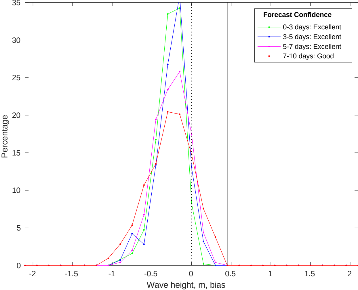
NDBC 52213 vs CMEMS Waves Bias Histogram: 14-Jan-2026
