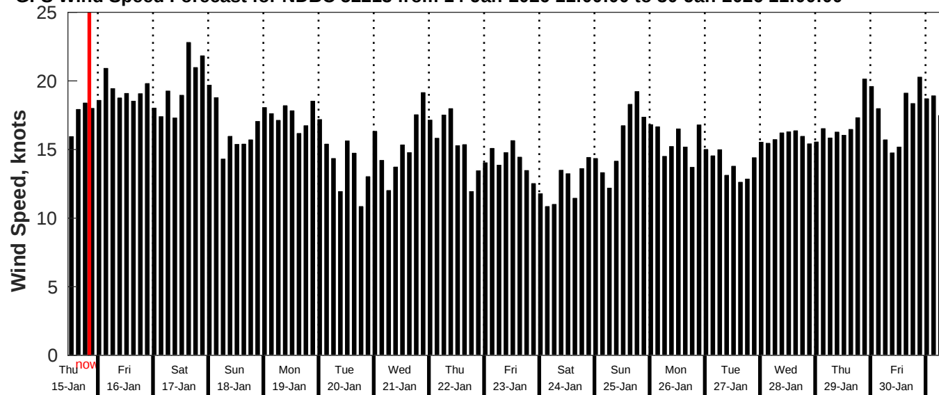
GFS Wind Speed Forecast for NDBC 52213 from 14-Jan-2026 11:00:00 to 30-Jan-2026 11:00:00
