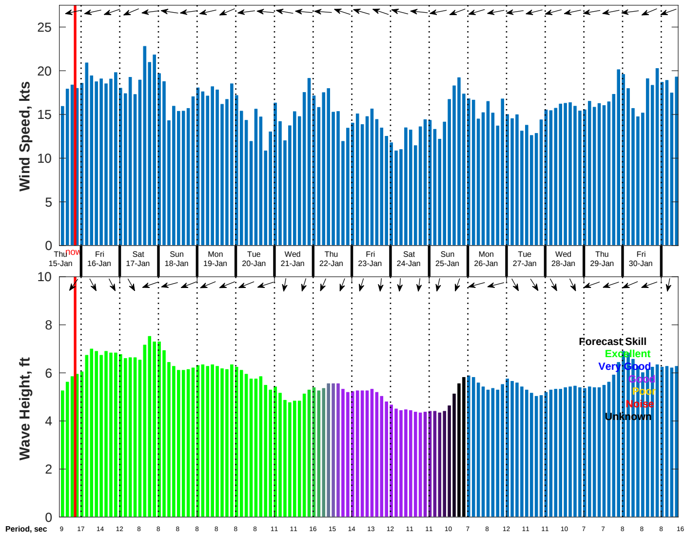
Wind & Wave Forecast for NDBC 52213 from 14-Jan-2026 11:00:00 to 30-Jan-2026 11:00:00
