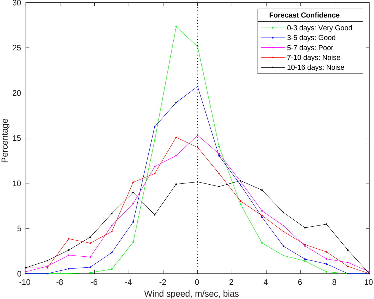
NDBC 41004 vs GFS Winds Bias Histogram: 15-Jan-2026
