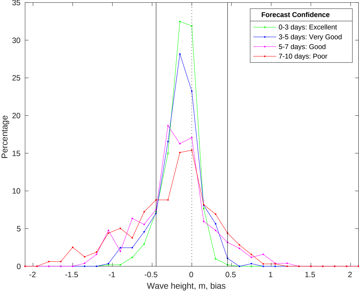
NDBC 41013 vs CMEMS Waves Bias Histogram: 15-Jan-2026
