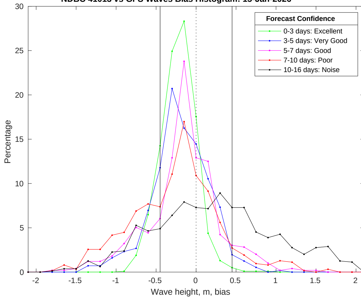
NDBC 41013 vs GFS Waves Bias Histogram: 15-Jan-2026
