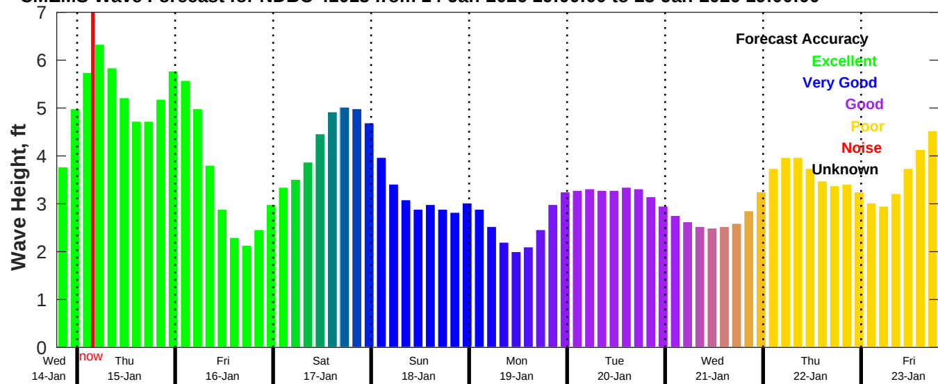
CMEMS Wave Forecast for NDBC 41013 from 14-Jan-2026 19:00:00 to 23-Jan-2026 19:00:00
