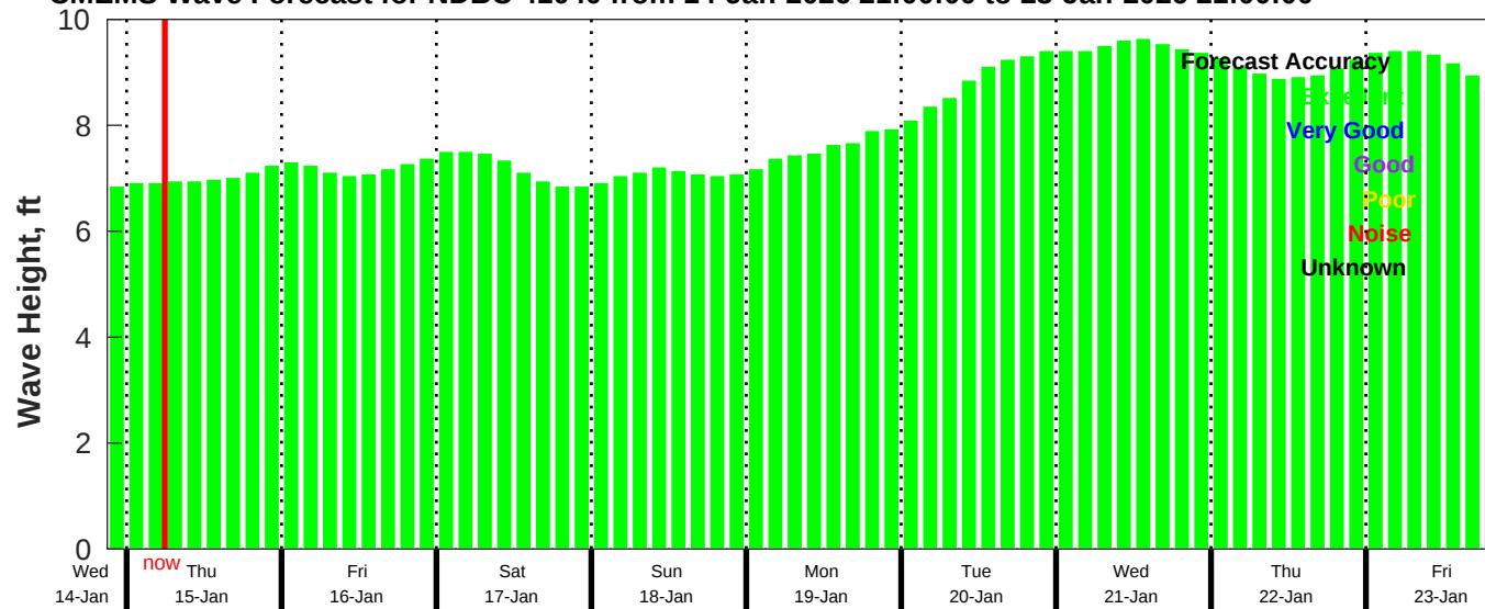
CMEMS Wave Forecast for NDBC 41040 from 14-Jan-2026 21:00:00 to 23-Jan-2026 21:00:00
