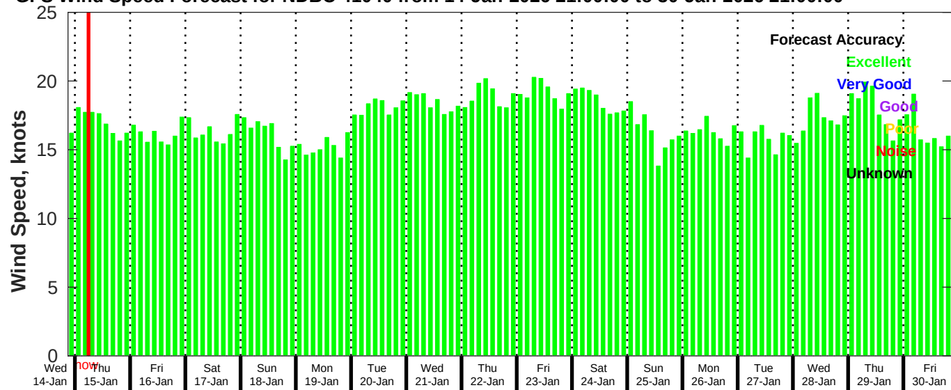
GFS Wind Speed Forecast for NDBC 41040 from 14-Jan-2026 21:00:00 to 30-Jan-2026 21:00:00
