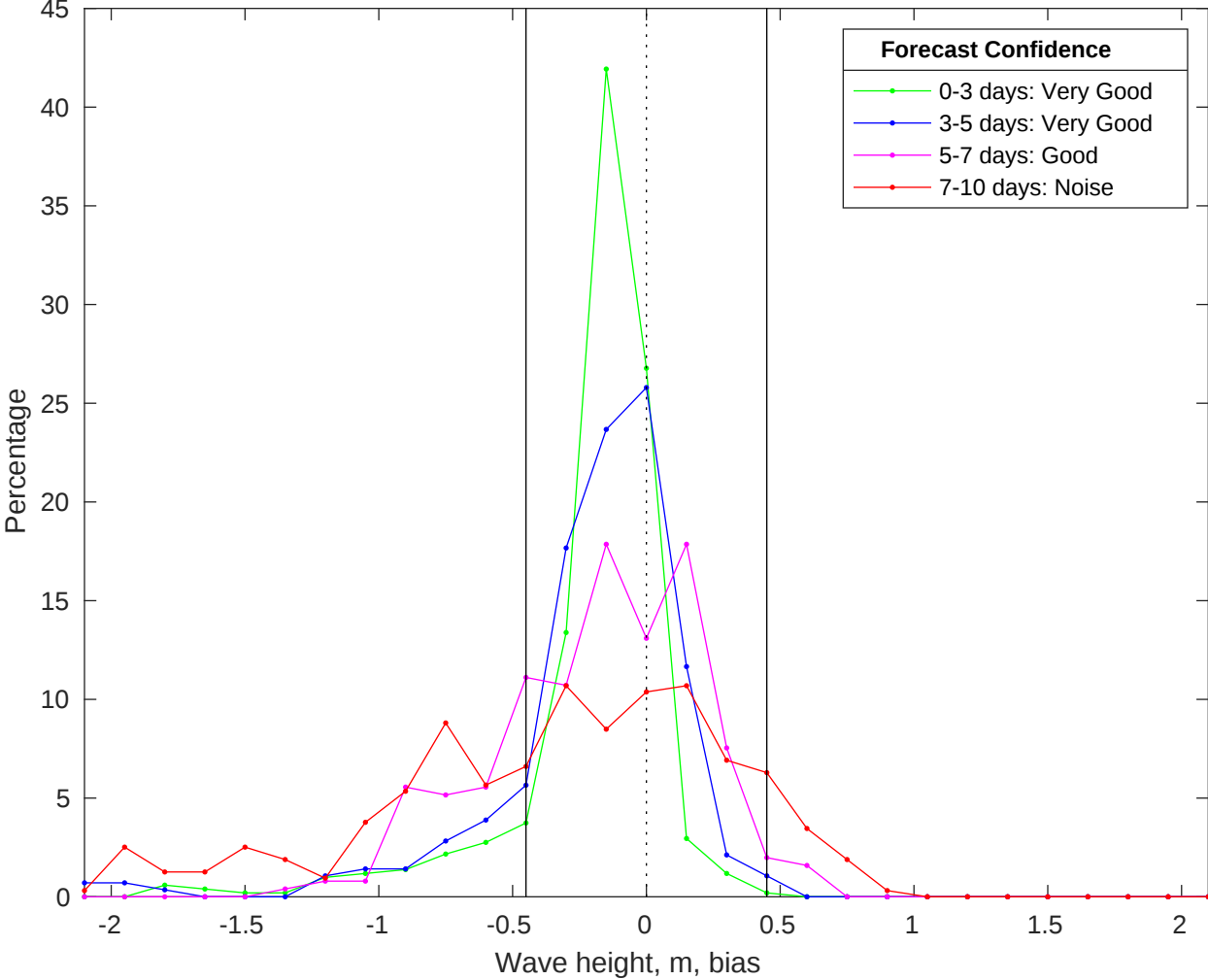
NDBC 42019 vs CMEMS Waves Bias Histogram: 15-Jan-2026
