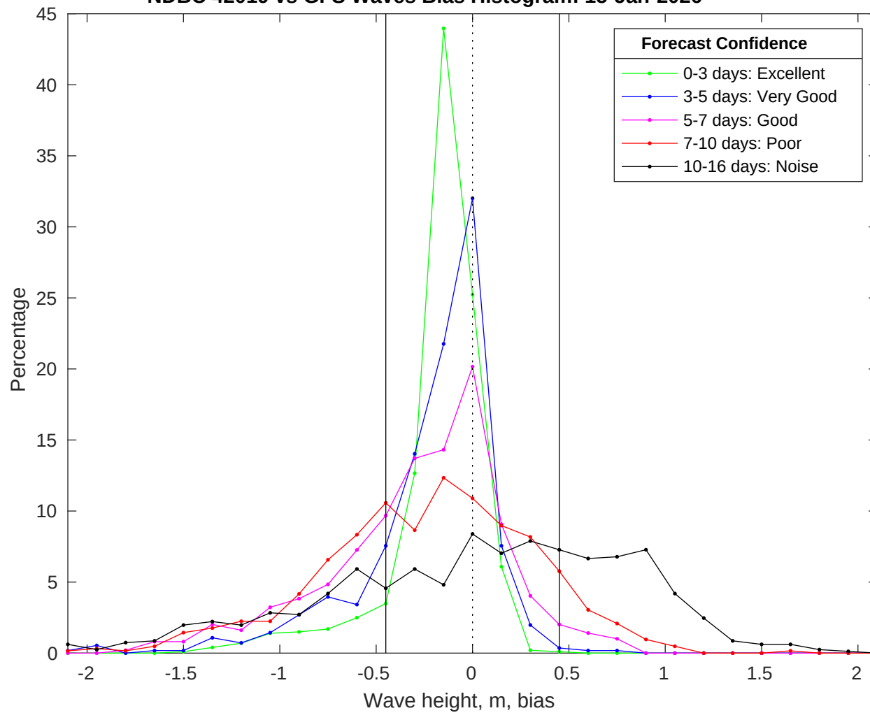
NDBC 42019 vs GFS Waves Bias Histogram: 15-Jan-2026
