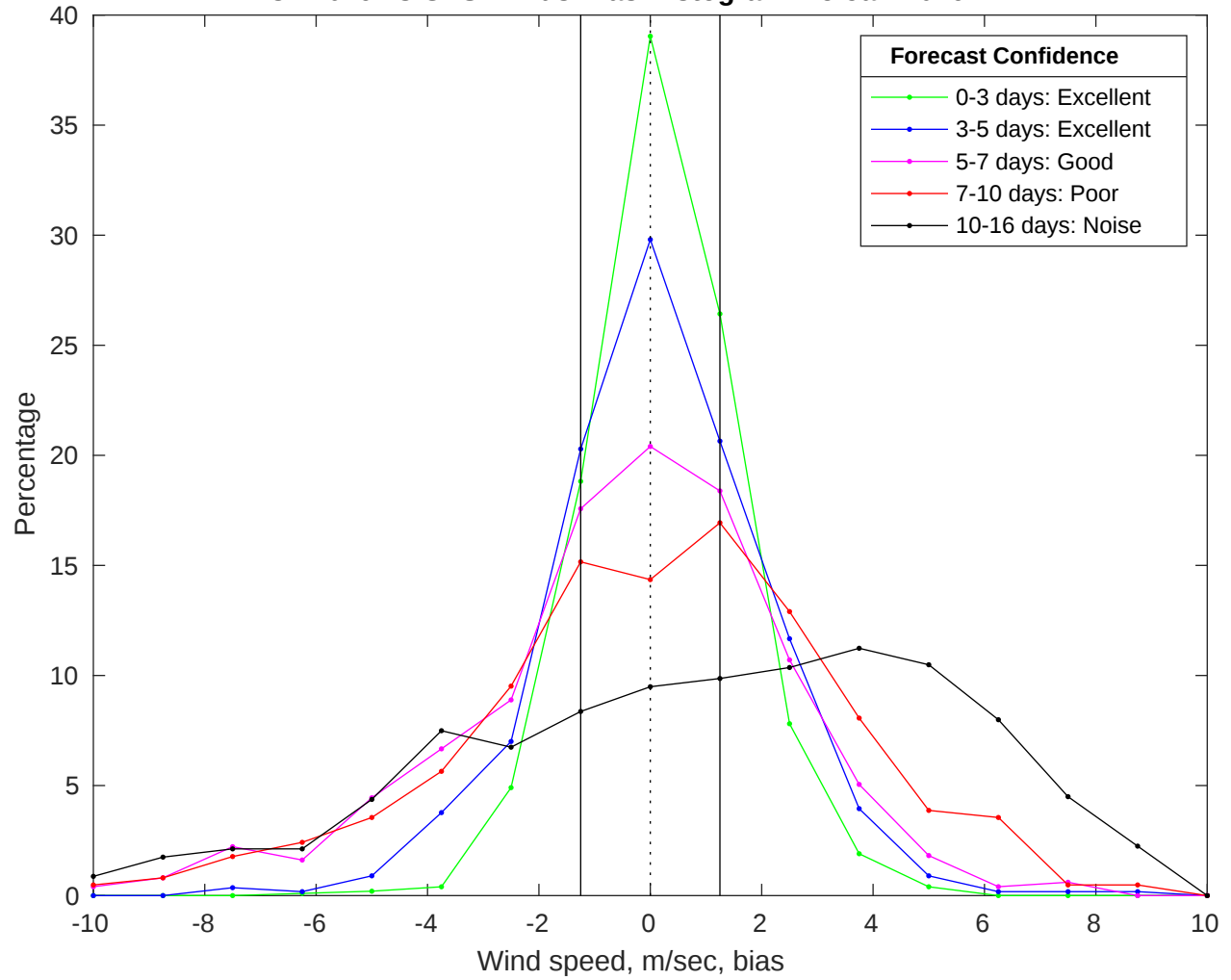
NDBC 42019 vs GFS Winds Bias Histogram: 15-Jan-2026
