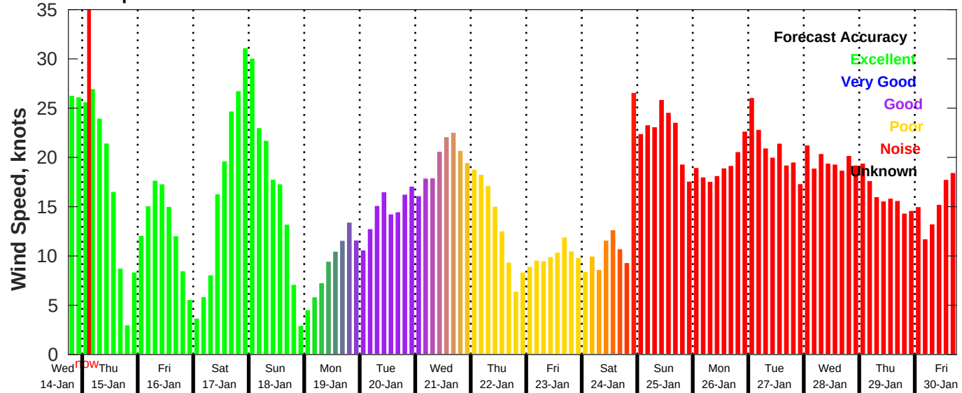
GFS Wind Speed Forecast for NDBC 42019 from 14-Jan-2026 18:00:00 to 30-Jan-2026 18:00:00
