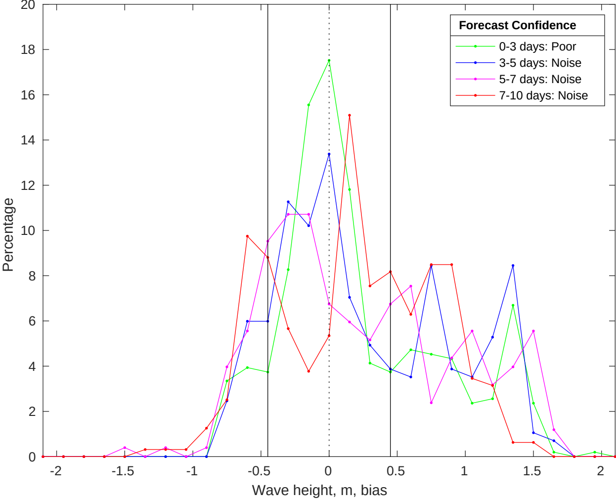
NDBC 42020 vs CMEMS Waves Bias Histogram: 15-Jan-2026
