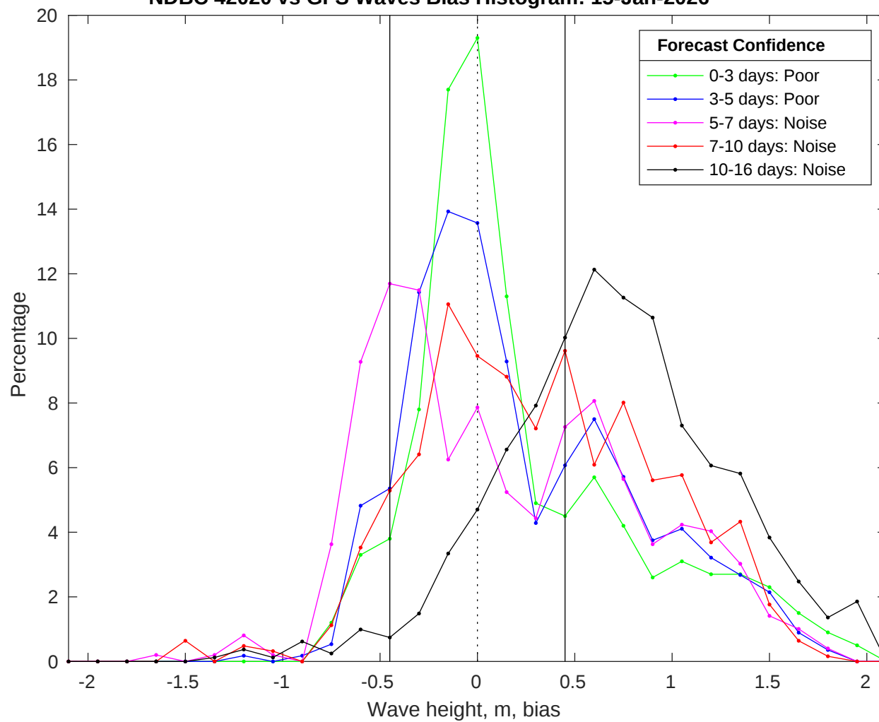
NDBC 42020 vs GFS Waves Bias Histogram: 15-Jan-2026
