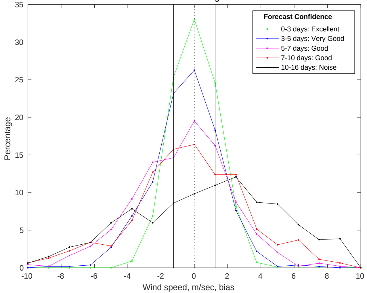
NDBC 42020 vs GFS Winds Bias Histogram: 15-Jan-2026
