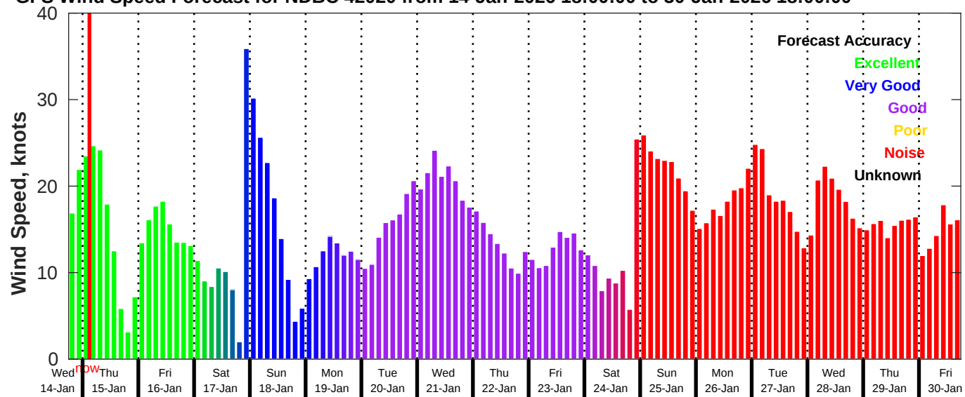
GFS Wind Speed Forecast for NDBC 42020 from 14-Jan-2026 18:00:00 to 30-Jan-2026 18:00:00
