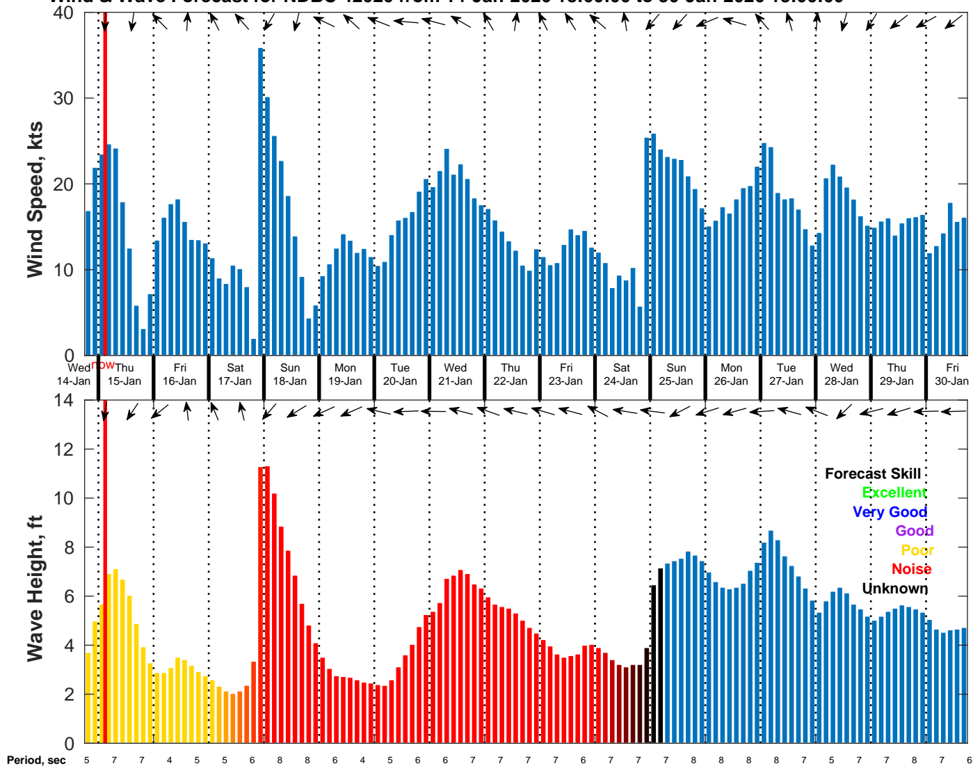
Wind & Wave Forecast for NDBC 42020 from 14-Jan-2026 18:00:00 to 30-Jan-2026 18:00:00
