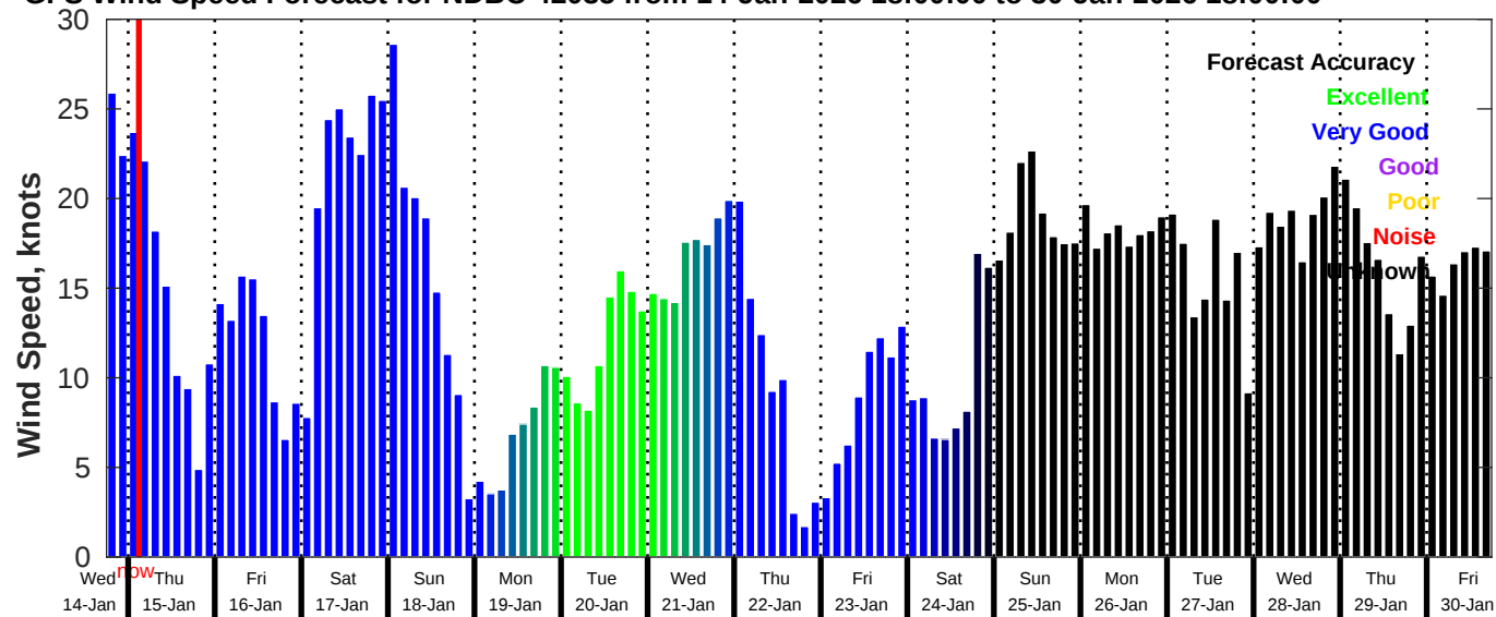
GFS Wind Speed Forecast for NDBC 42035 from 14-Jan-2026 18:00:00 to 30-Jan-2026 18:00:00
