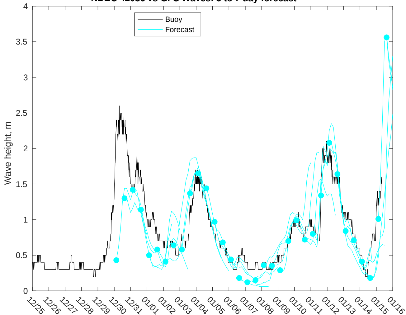
NDBC 42036 vs GFS Waves: 5 to 7 day forecast
