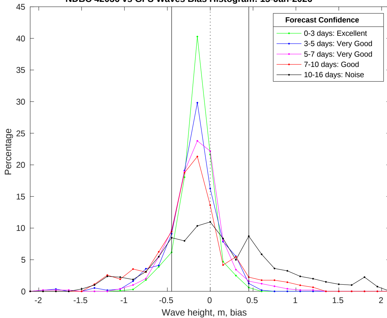
NDBC 42036 vs GFS Waves Bias Histogram: 15-Jan-2026
