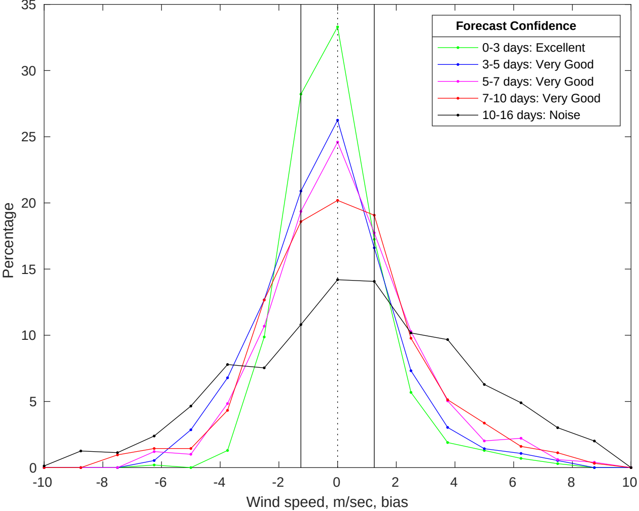
NDBC 42036 vs GFS Winds Bias Histogram: 15-Jan-2026
