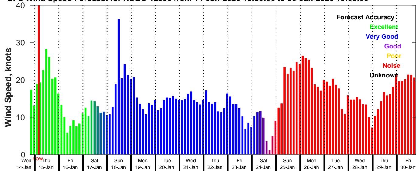
GFS Wind Speed Forecast for NDBC 42036 from 14-Jan-2026 19:00:00 to 30-Jan-2026 19:00:00
