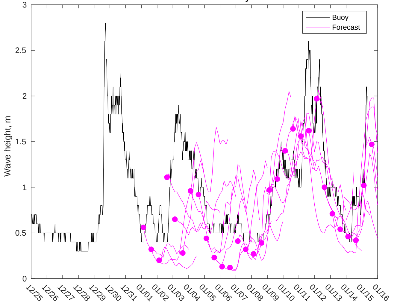
NDBC 42040 vs GFS Waves: 7 to 10 day forecast
