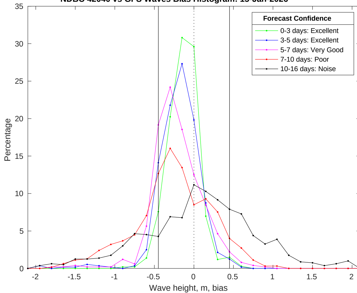
NDBC 42040 vs GFS Waves Bias Histogram: 15-Jan-2026
