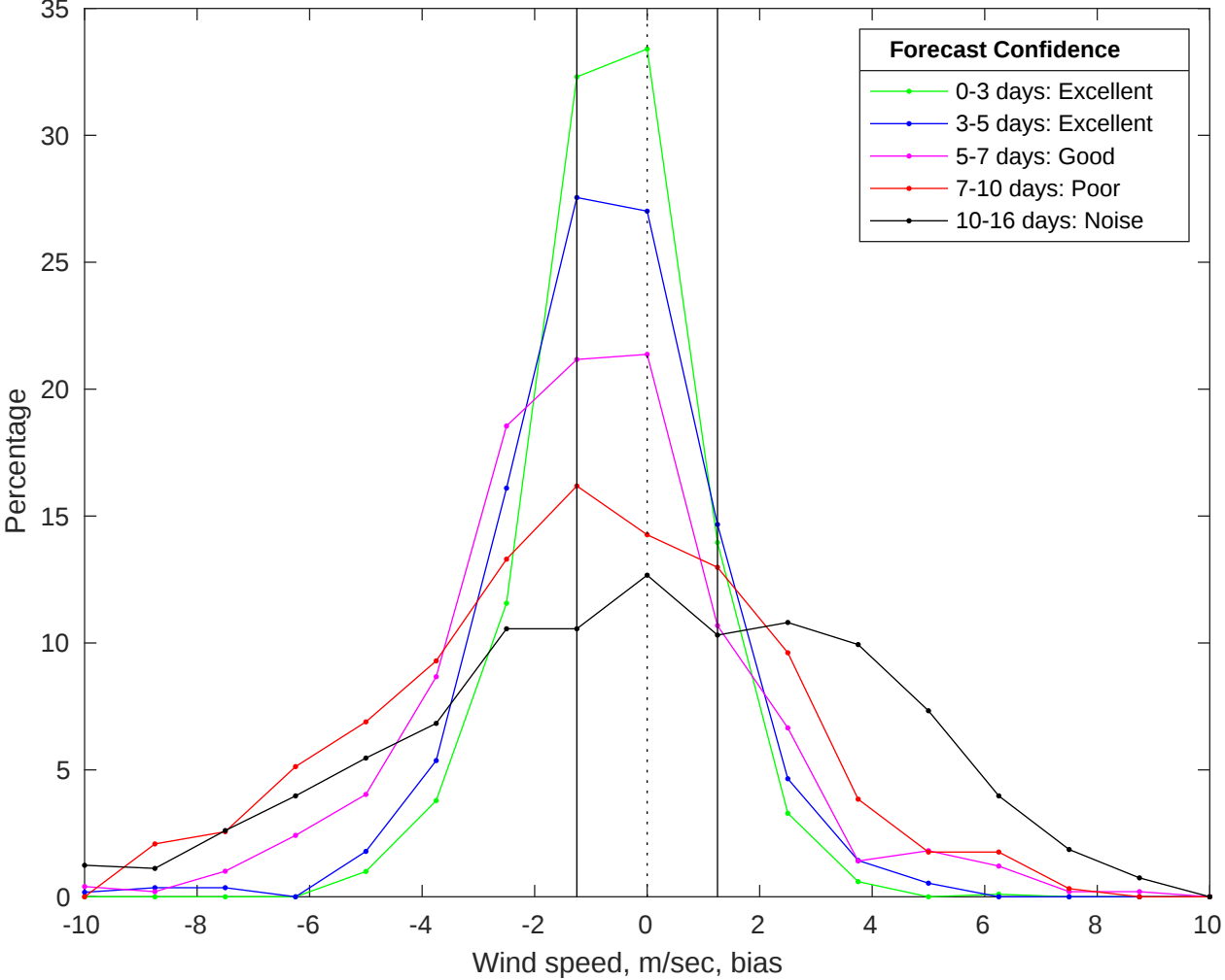
NDBC 42040 vs GFS Winds Bias Histogram: 15-Jan-2026
