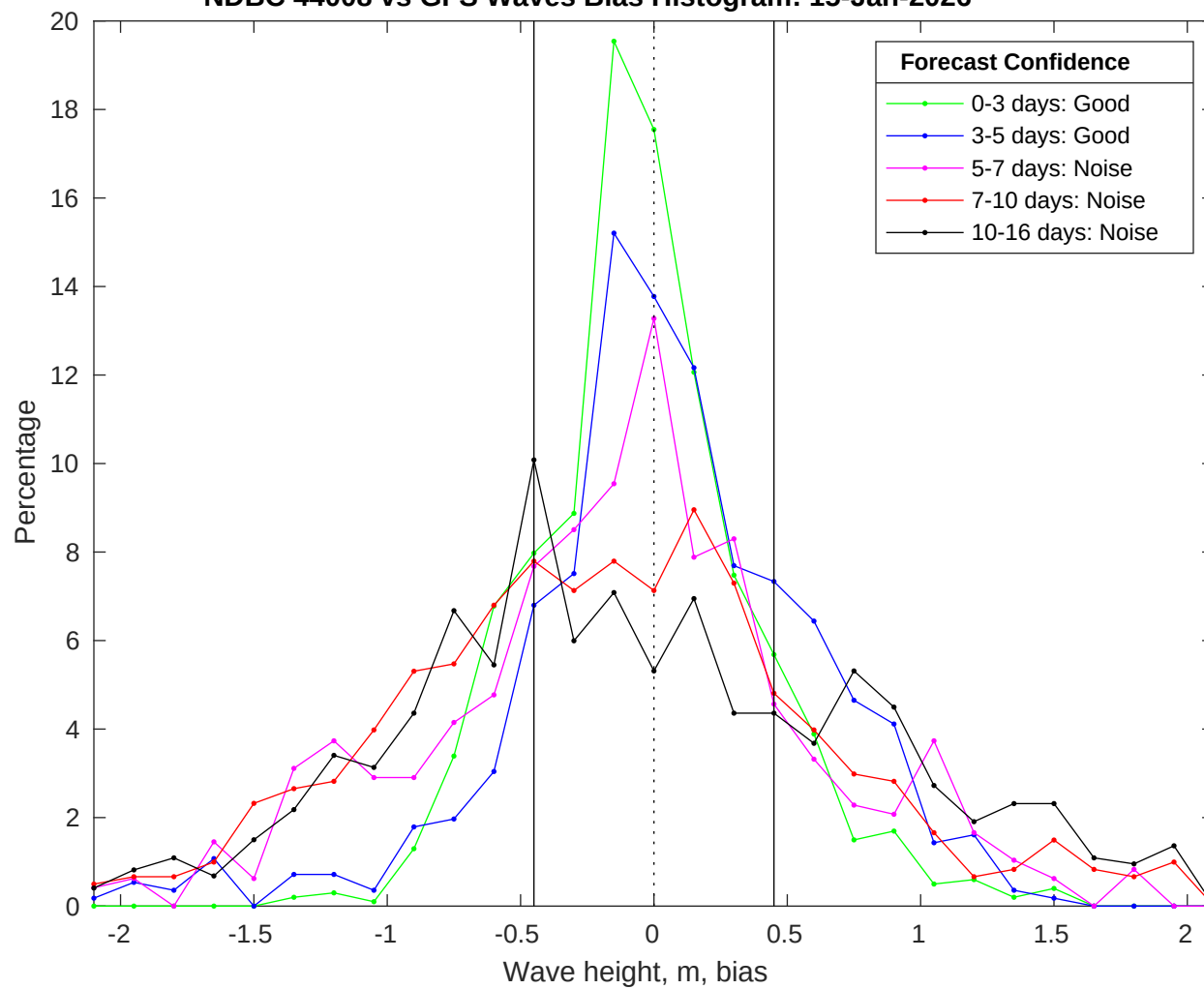
NDBC 44008 vs GFS Waves Bias Histogram: 15-Jan-2026
