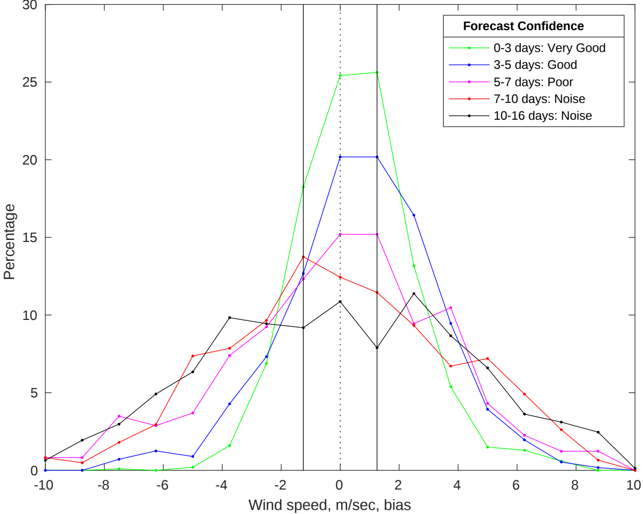
NDBC 44008 vs GFS Winds Bias Histogram: 15-Jan-2026
