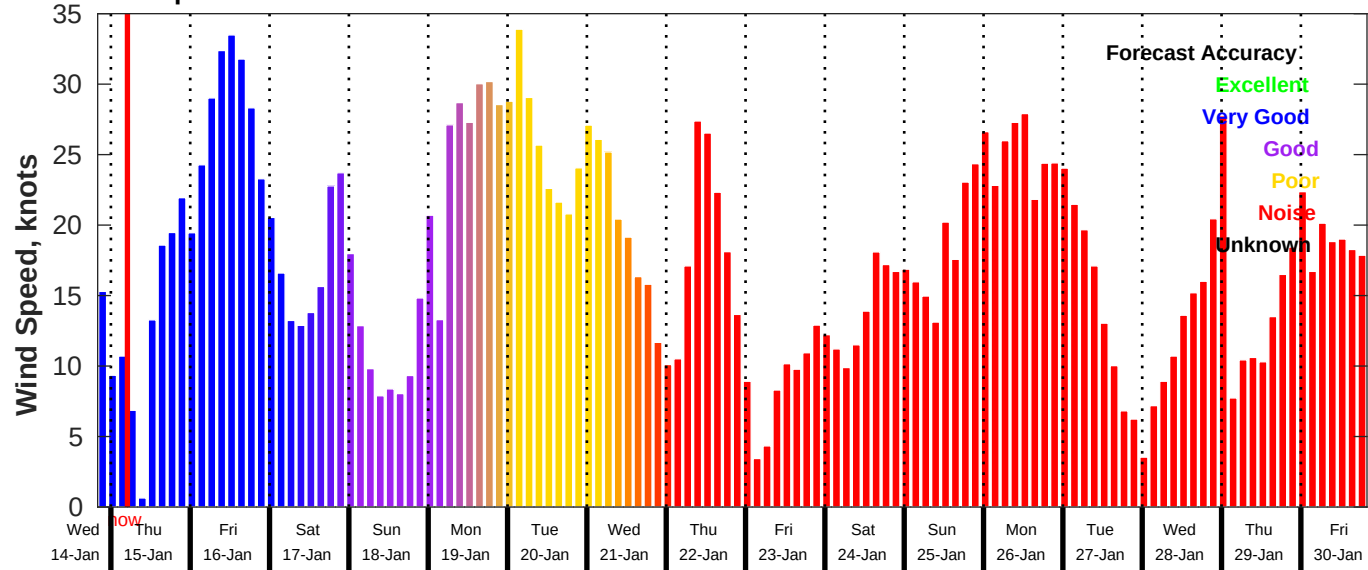
GFS Wind Speed Forecast for NDBC 44008 from 14-Jan-2026 20:00:00 to 30-Jan-2026 20:00:00
