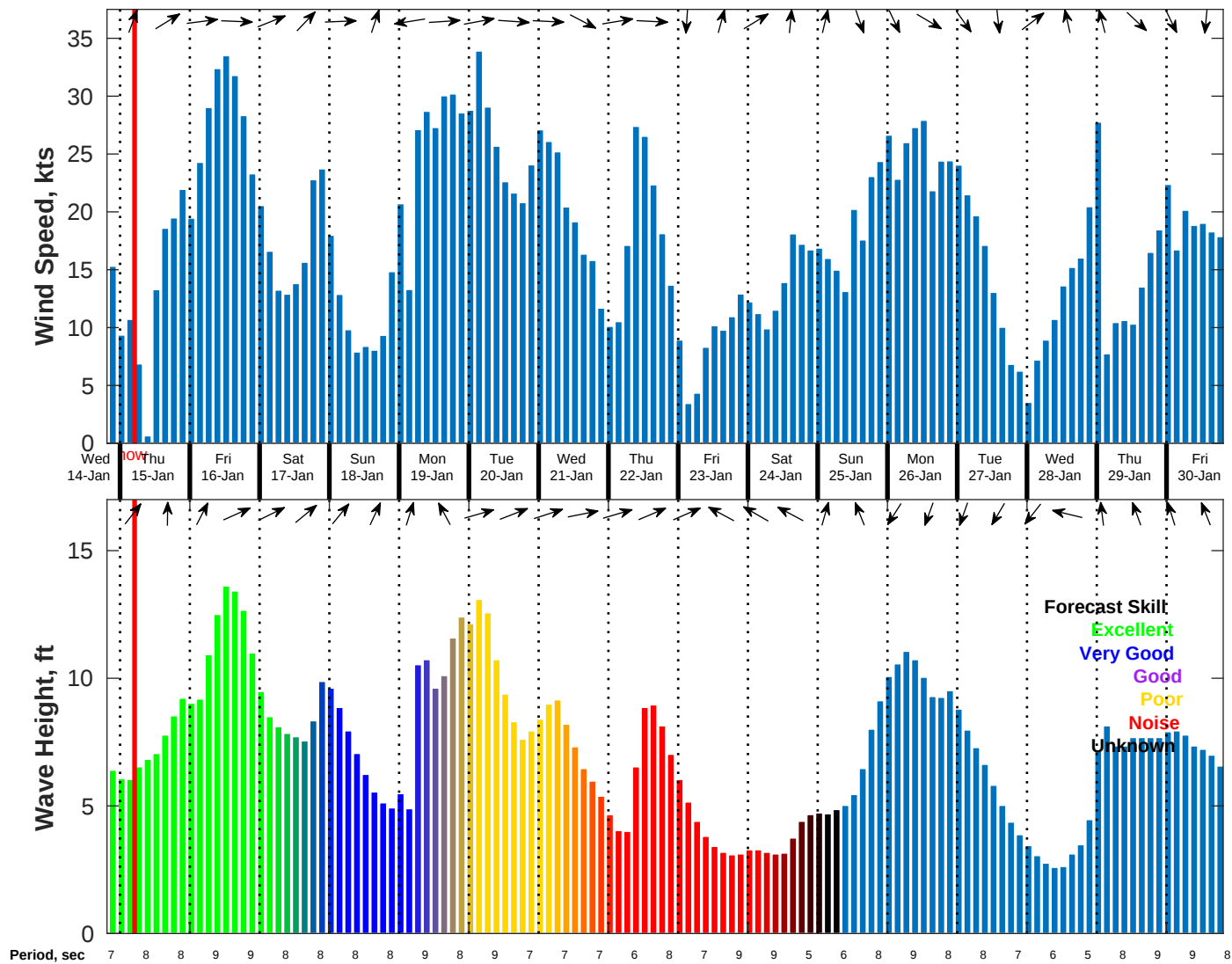
Wind & Wave Forecast for NDBC 44008 from 14-Jan-2026 20:00:00 to 30-Jan-2026 20:00:00
