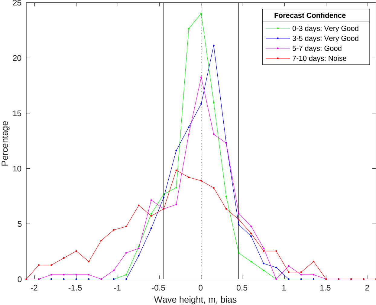
NDBC 46011 vs CMEMS Waves Bias Histogram: 15-Jan-2026
