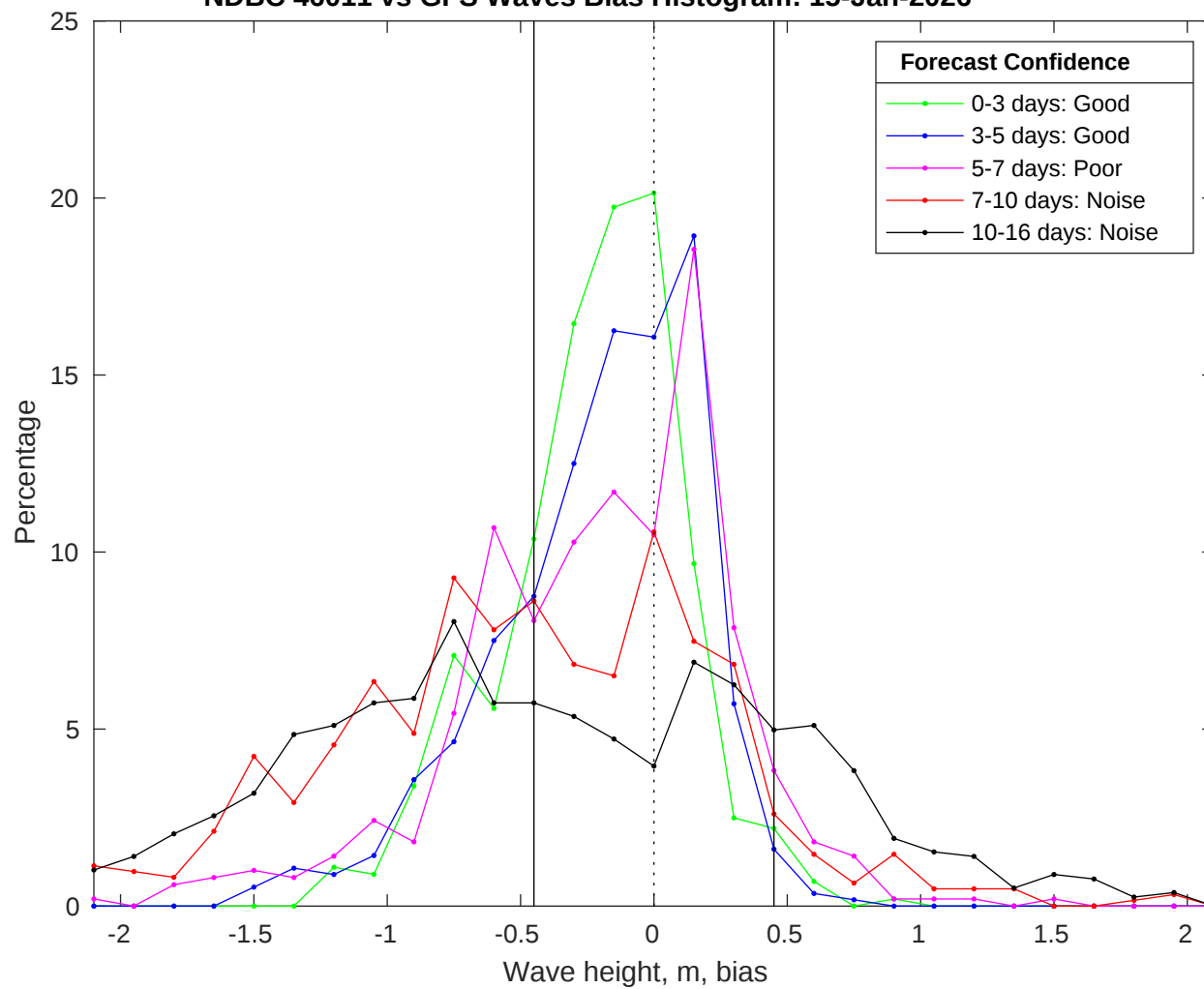
NDBC 46011 vs GFS Waves Bias Histogram: 15-Jan-2026
