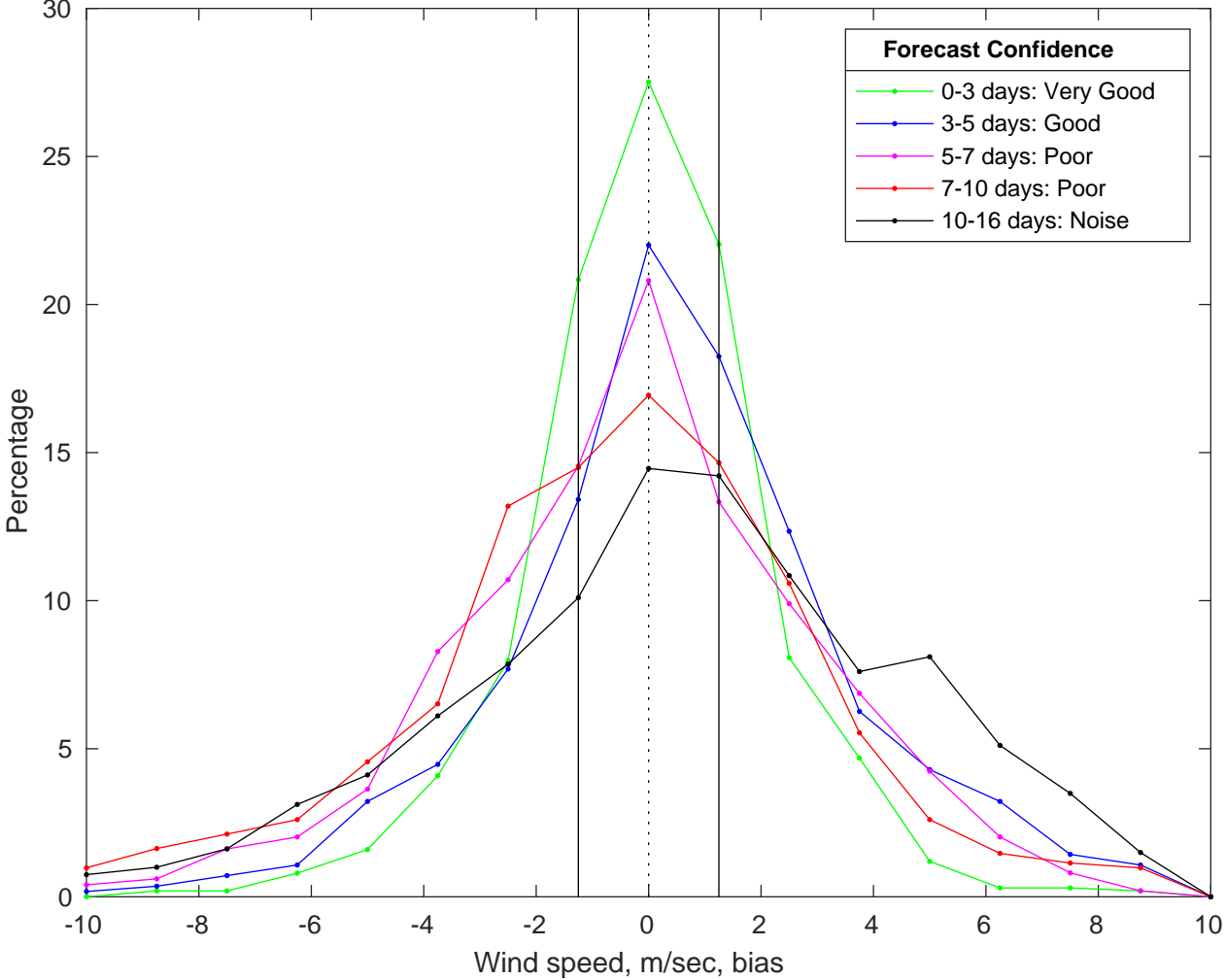
NDBC 46011 vs GFS Winds Bias Histogram: 15-Jan-2026
