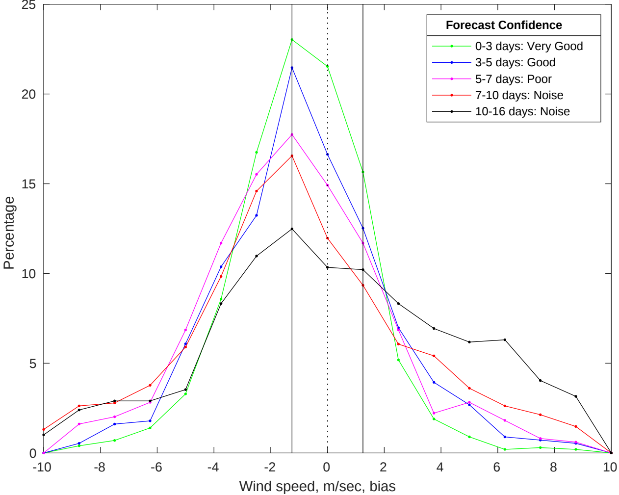
NDBC 46028 vs GFS Winds Bias Histogram: 15-Jan-2026
